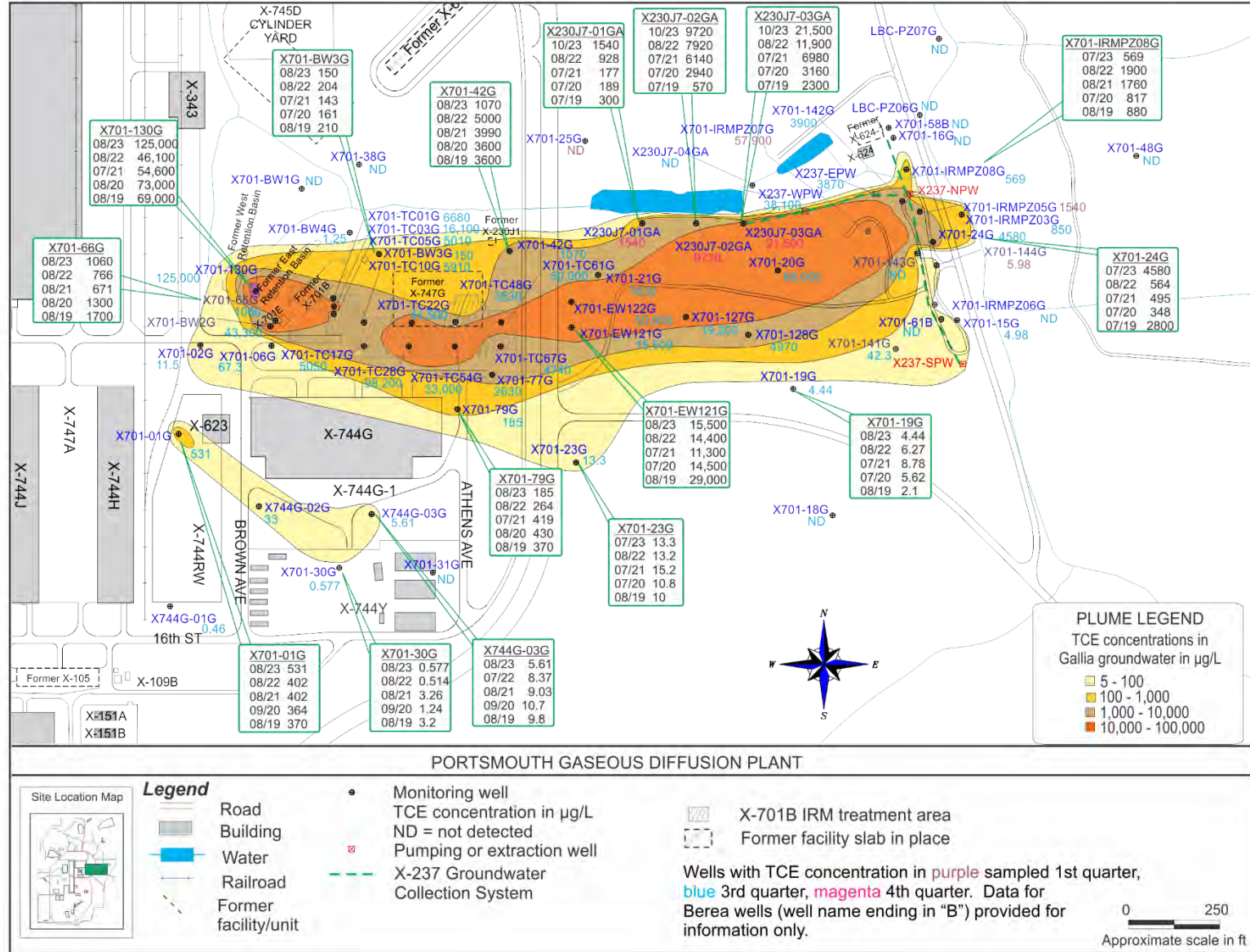
Figure 6.5. Gallia groundwater plume contaminated with trichloroethene at the X-701B Former Holding Pond in 2023
