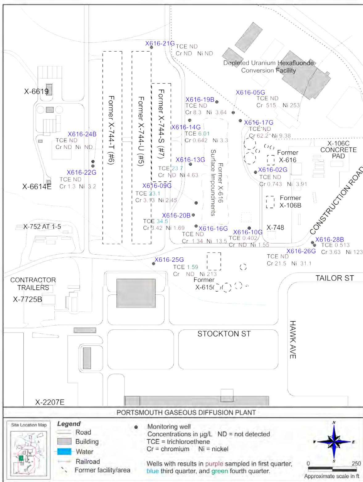
Figure 6.6. Trichloroethene and metal concentrations in groundwater at the X-616 Former Chromium Sludge Surface Impoundments in 2023
