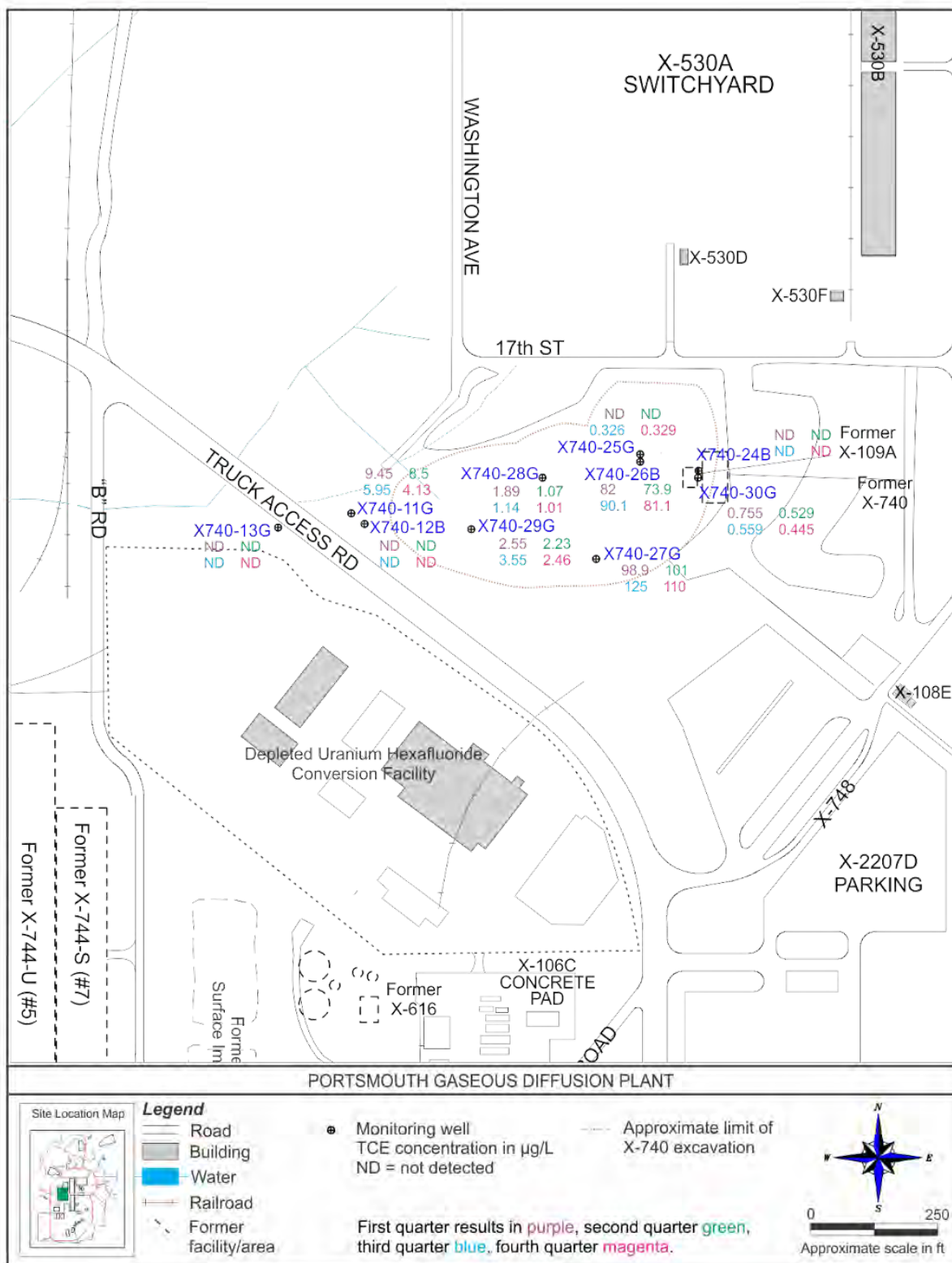
Figure 6.7. Trichloroethene concentrations in groundwater at the X-740 Former Waste Oil Handling Facility in 2023
