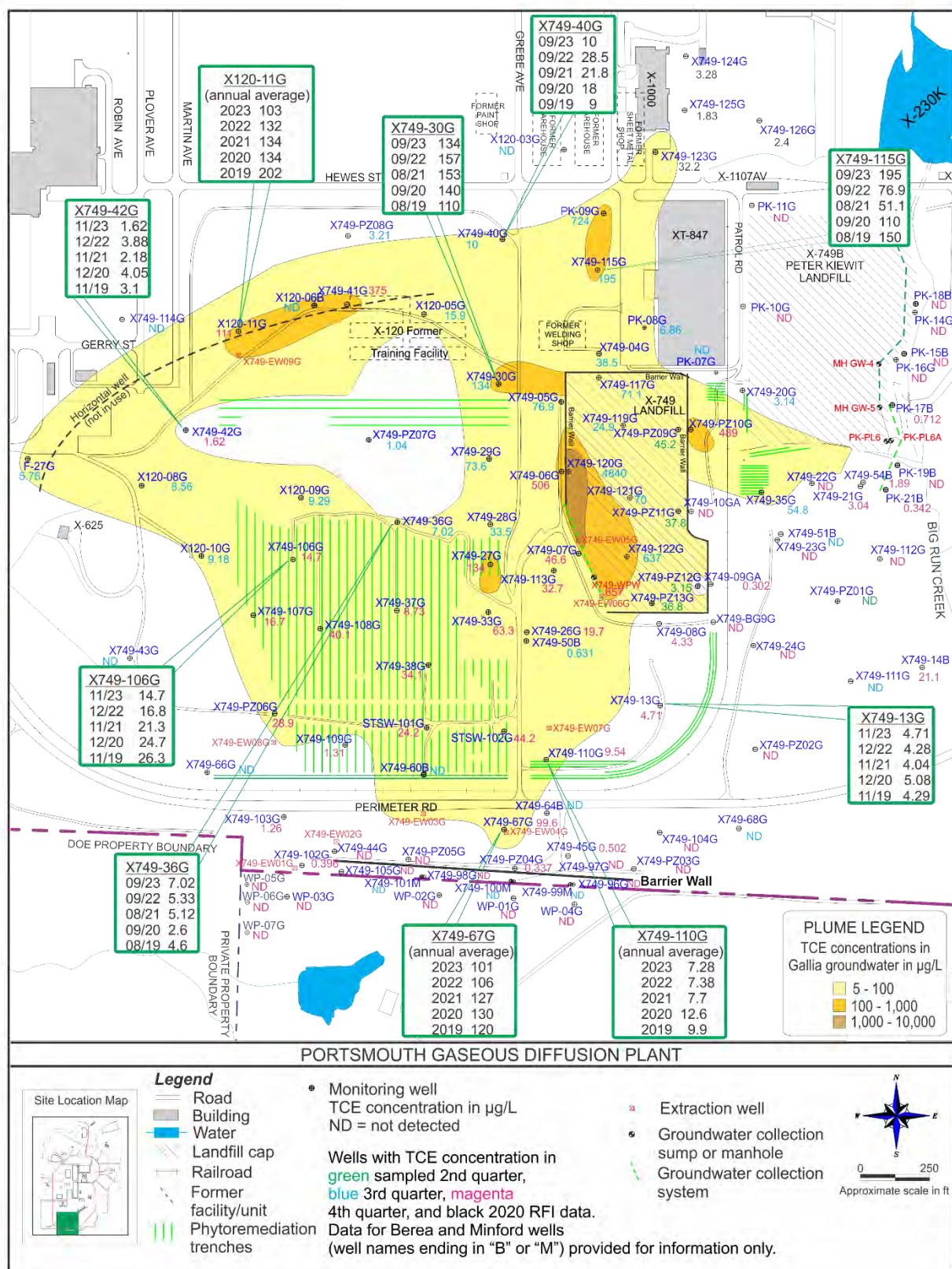
Figure 6.2. Gallia groundwater plume contaminated with trichloroethene at the X-749 Contaminated Materials Disposal Facility/X-120 Former Training Facility in 2023
